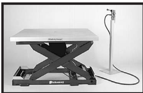
EZU-15-R with optional 48" x 48" rotating top and pedestal valve stand
