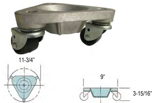
MODEL 2127 AL
