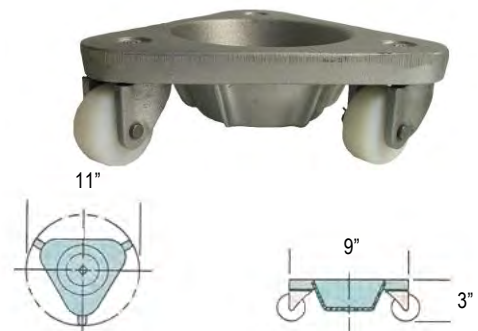
MODEL 2127 AL
